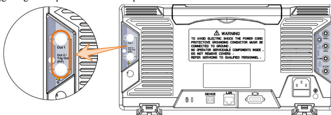
Figure 5-1 Generator Output Ports (Dual-channel)
