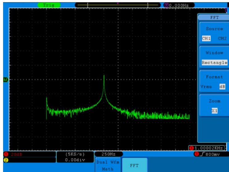
Fig. 20 Rectangle window
