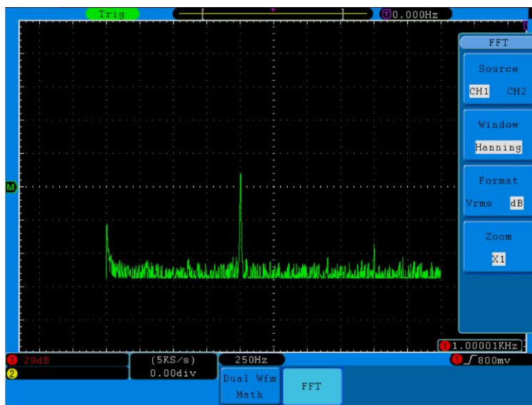
Fig. 22 Hanning window
