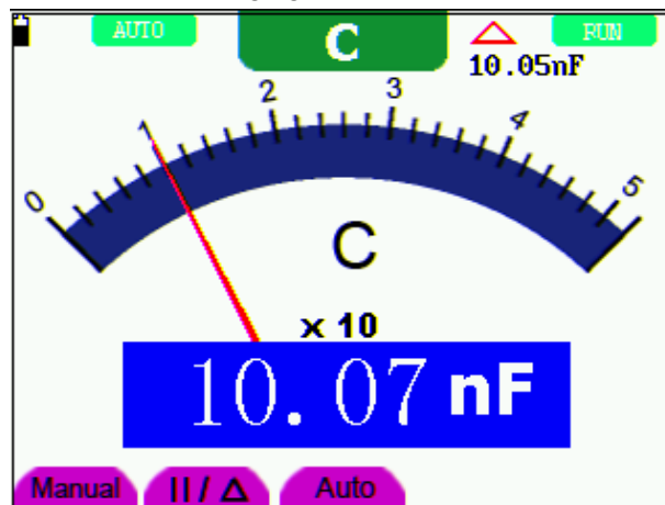
Figure 20: Capacitance Measurement
