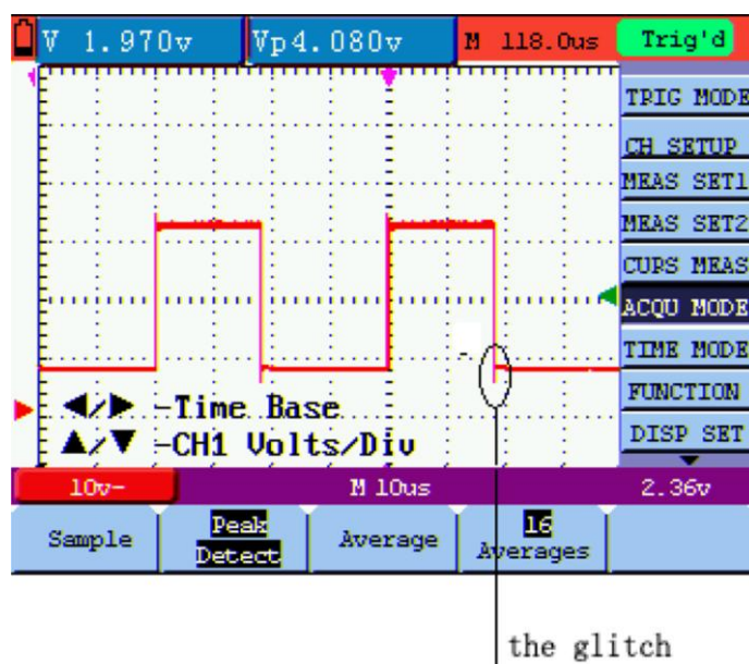
Figure 13: Peak Detection
